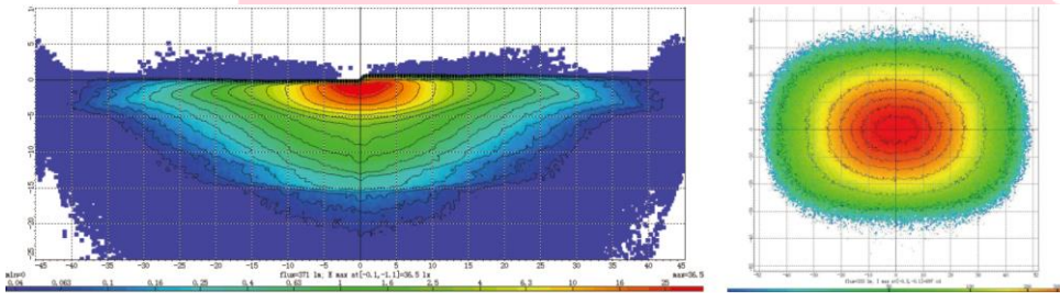
Low beam head light
